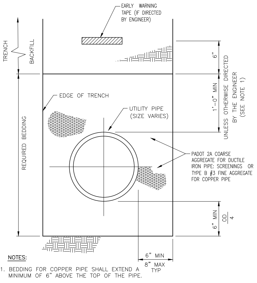
STANDARD PIPE BEDDING NOT TO SCALE
