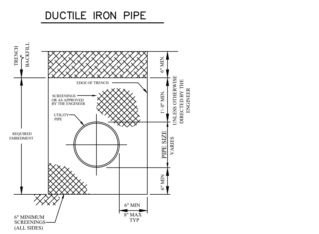
DUCTILE IRON PIPE COPPER PIPE PIPE EMBEDMENT NOT TO SCALE
